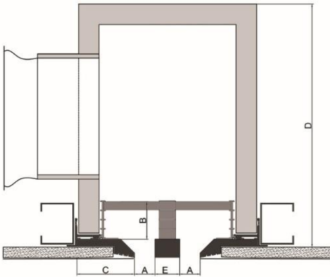
INVI LINE 2+ SECTION
